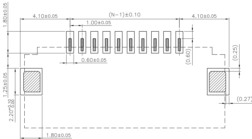
PCB LAYOUT
