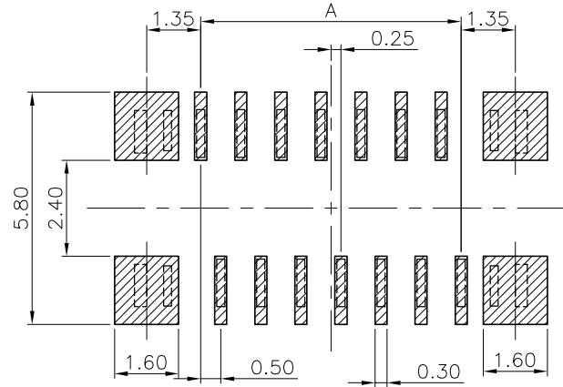
PCB LAYOUT(反脚)
