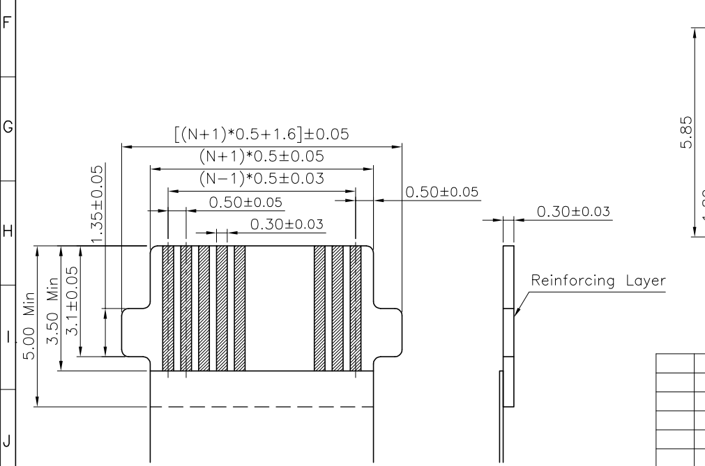
RECOMMENDED FFC/FPC DIMENSION
